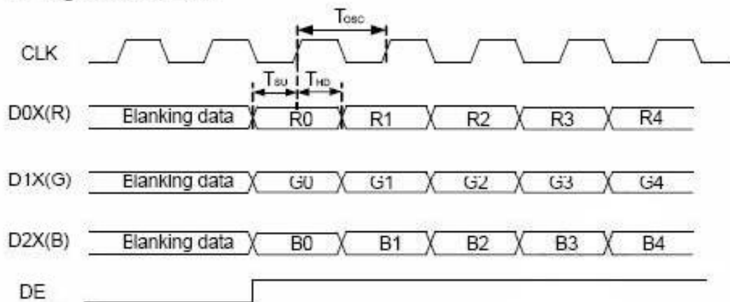
Figure4 CLK,DATA and DE wavedforms in Digital Parallel RGB
