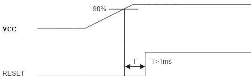
Reset timing
