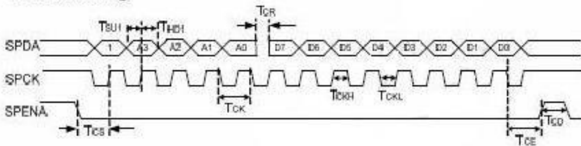
Figure8 SPI read timing
