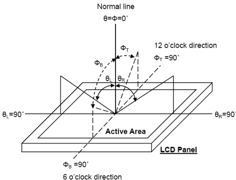
Fig. 8-1 Definition of viewing angle
