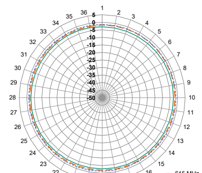
XY-Plane Gain
