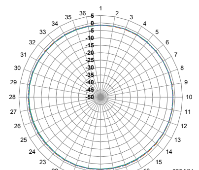
XY-Plane Gain
